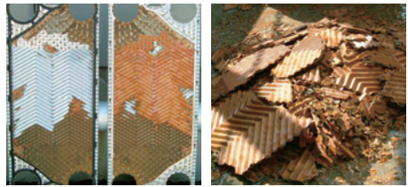
↑ Hard scale inside the plates
