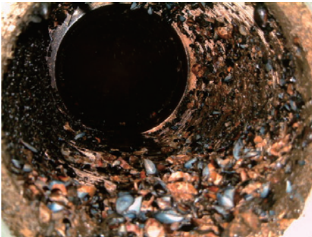
↑ Heat exchanger Seawater inlet port hole Wood chips, seaweeds and shellfish are blocking the flow channel, and causing poor flow in the unit.
